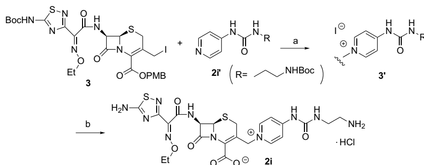
Scheme 1. Reagents and conditions: (a) 2i' , MeCN, rt, 90 min; (b) (i) AlCl 3 -anisole, CH 2 Cl 2 , –40–0 °C, (ii) purification by HP-20 chromatography.
